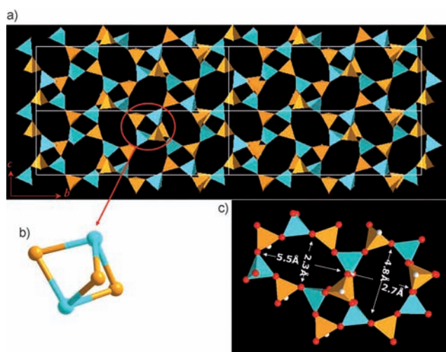
Figure 2. a) Inorganic layer viewed along [100]. b) Ball-and-stick representation of the 4=1 SBU. Oxygen atoms are omitted for clarity and sticks represent the T–O bonds. c) Polyhedral representation of the two 8MRs of the inorganic layer. Al turquoise, Si yellow, C white, O red.
